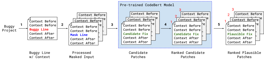
Figure 2: AlphaRepair overview
