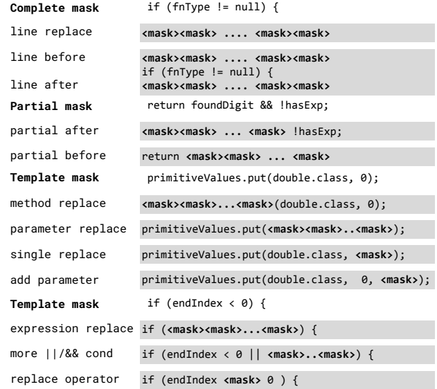
Figure 4: Different strategies to generate mask lines
